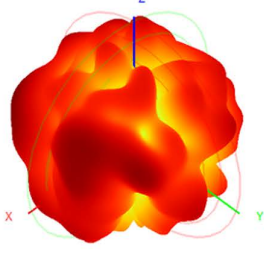
5750.0MHz H+V, Eff. 30.9%
