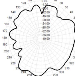
Total(H-XY), Max= -0.45dB, CirD=16.92
