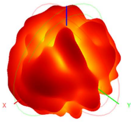
5550.0MHz H+V, Eff. 30.6%
