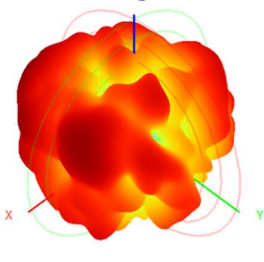
5950.0MHz H+V, Eff. 31.2%
