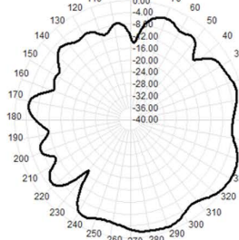
Total(H-XY), Max= 0.70dB, CirD=17.77
