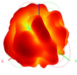
5450.0MHz H+V, Eff. 30.4%
