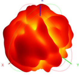
5650.0MHz H+V, Eff. 29.6%
