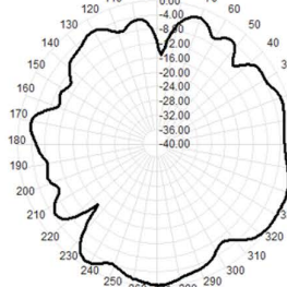
Total(H-XY), Max= -0.35dB, CirD=15.97
