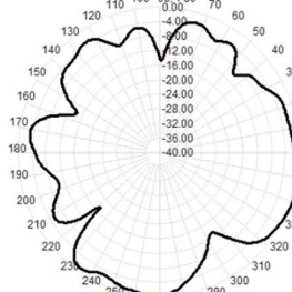
Total(H-XY), Max= -0.48dB, CirD=17.49
