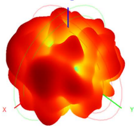
5850.0MHz H+V, Eff. 31.4%
